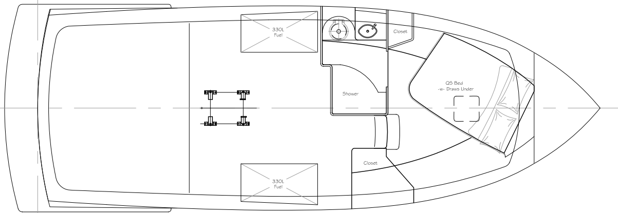
Accommodation Deck Plan
